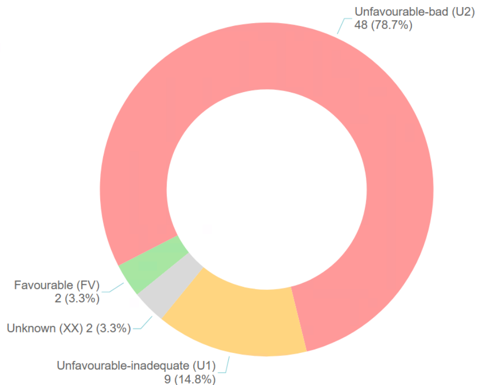
Figure 3.3 Overall conservation status of habitats in Wales (2019-2024 reporting).
